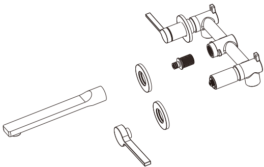
Faucet Body
