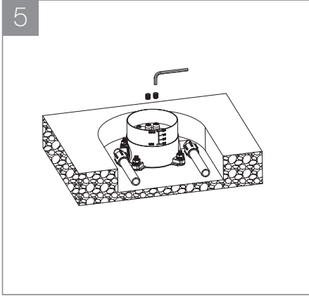
5. Use a hex wrench to unscrew the 2 gravel drain bolts inside the leak test plastic plug.
