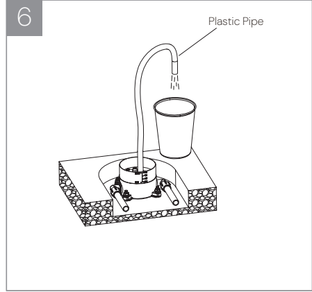
6. Prepare a bucket, insert the plastic tube into the top of the leak test plastic plug, then open the corresponding inlet valves one by one to drain the gravel and dirt remaining in the pipes.
