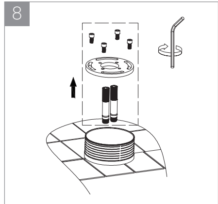
8. Remove the plate and plug by hexagon screw.
