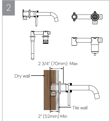
2. The installation depth of rough-in valve should be no less than 2" (52mm) and no more than 2 3/4" (70mm), including the thickness of tile. Otherwise the deck plate cannot be installed.
