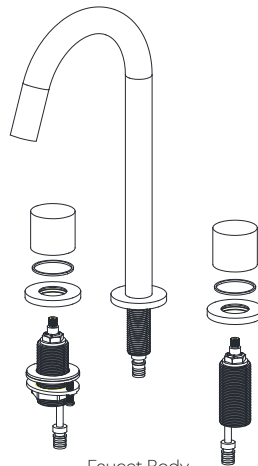
Faucet Body
