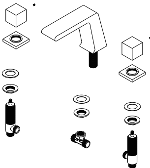
Faucet Body
