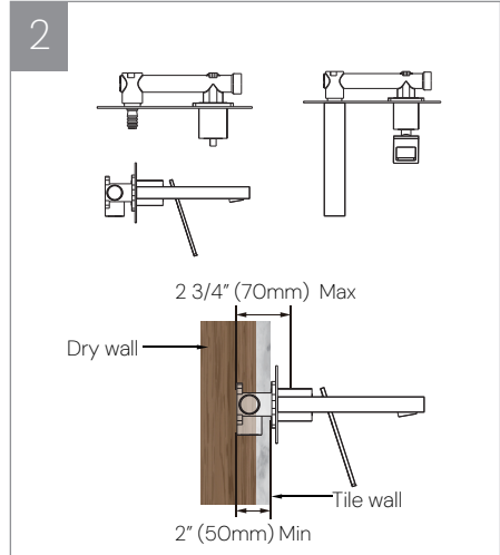
2. The installation depth of rough-in valve should be no less than 2" (50mm) and no more than 2 3/4" (70mm), including the thickness of tile. Otherwise the escutcheon cannot be installed.
