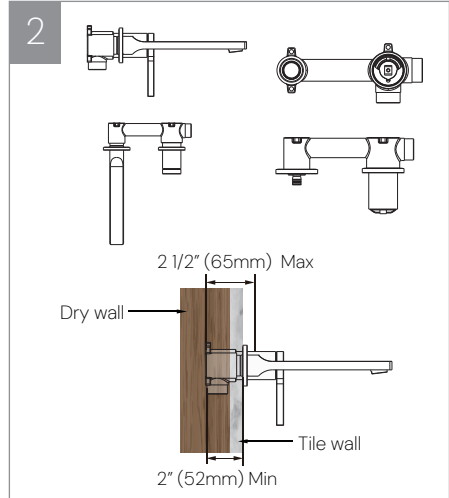
2. The installation depth of rough-in valve should be no less than 2" (52mm) and no more than 2 1/2" (65mm), including the thickness of tile. Otherwise the deck plate cannot be installed.
