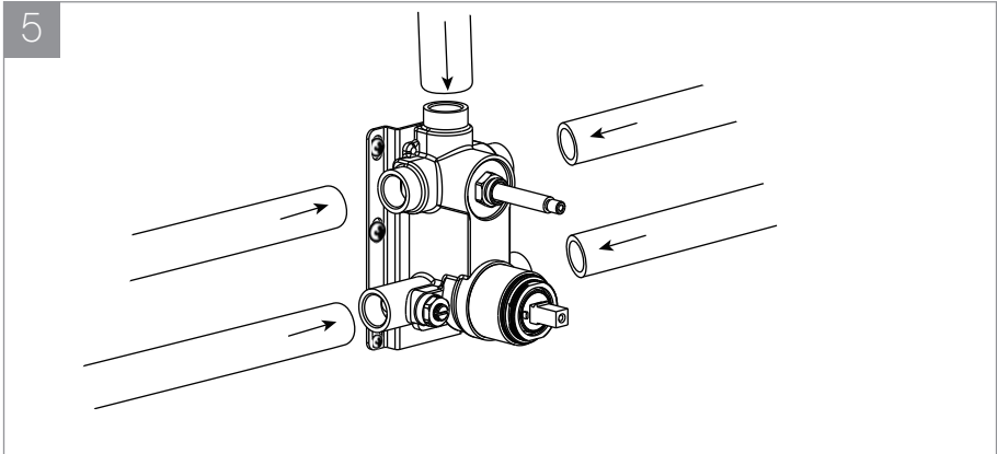
5. Connect the water pipe to the rough-in valve.
