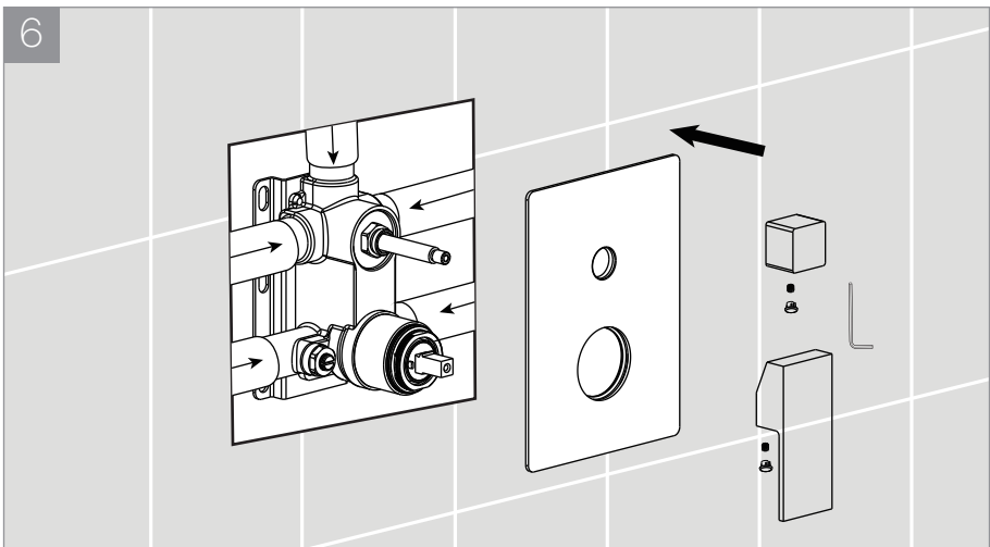
6. Align the escutcheon with the rough-in valve and securely install the knobs.
