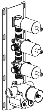
Rough-in Valve
